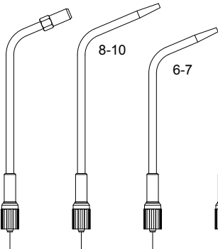
Style 760 Universal Heating Tip Assemblies Size 5 to 10
